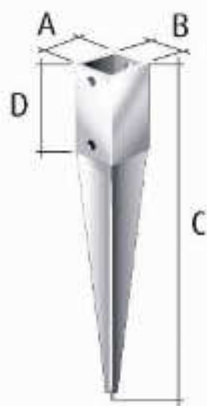
Square Post Anchor
